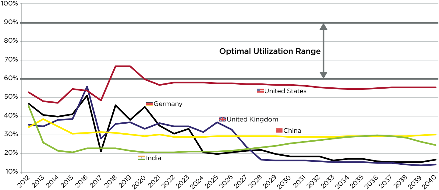
12 Figure 5: Historical and Projected Average Utilization Rates for CCGT Plants in Select Countries in BAU Scenario
